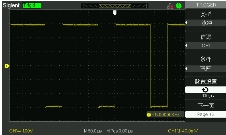
2-22 脉冲触发功能菜单 1
