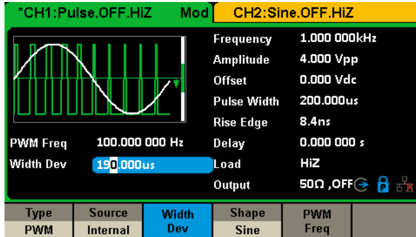
Figure 2-31 Setting Interface of PWM Modulation
