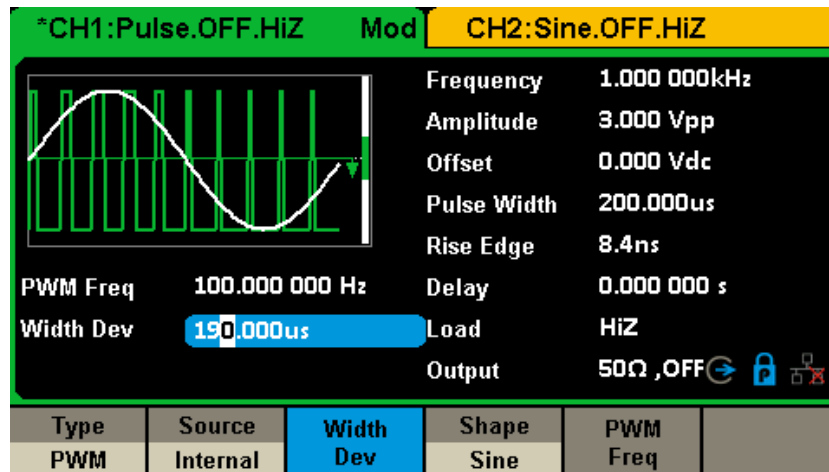
Figure 2-32 Width Deviation Setting Interface
