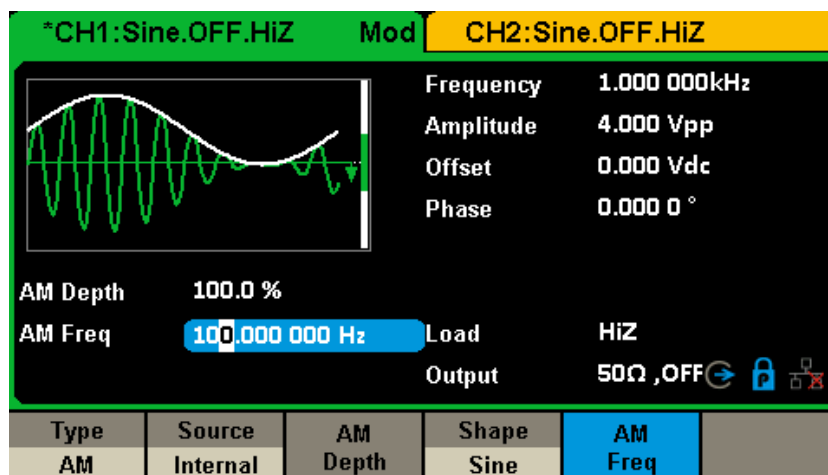
Figure 2-24 Setting Interface of AM Modulation
