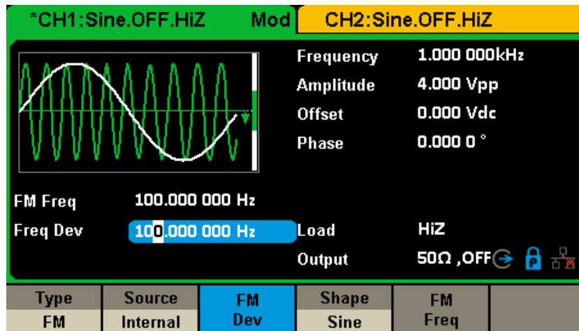
Figure 2-26 Setting Interface of FM Modulation
