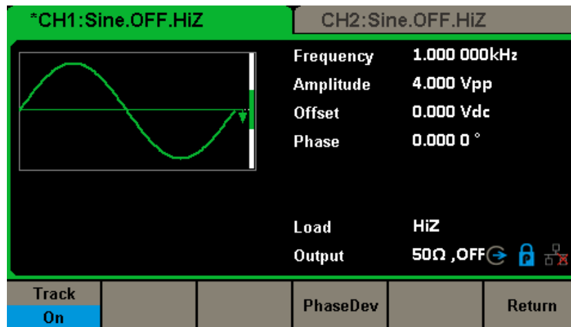
Figure 2-74 Track Interface
