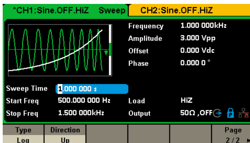
Figure 2-37 Log Sweep Interface
