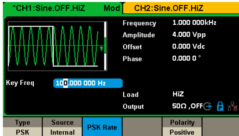
Figure 2-30 Setting Interface of PSK Modulation
