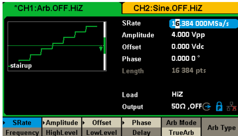
Figure 2-19 Arb Parameters Display Interface (TrueArb)
