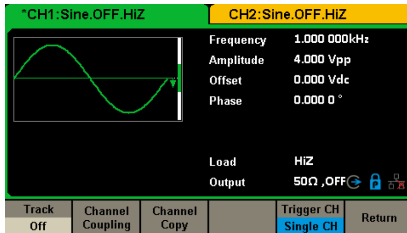
Figure 2-76 Channel trigger signal independent
