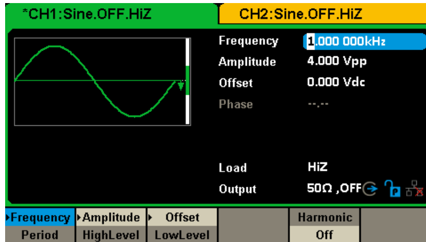
Figure 2-84 Independent Mode
