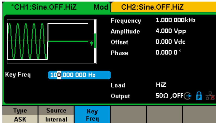
Figure 2-29 Setting Interface of ASK Modulation
