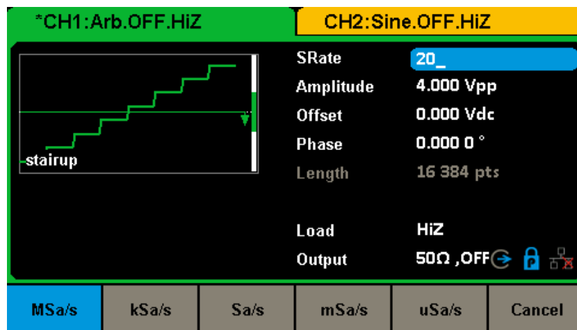
Figure 2-20 Setting the Sampling Rate
