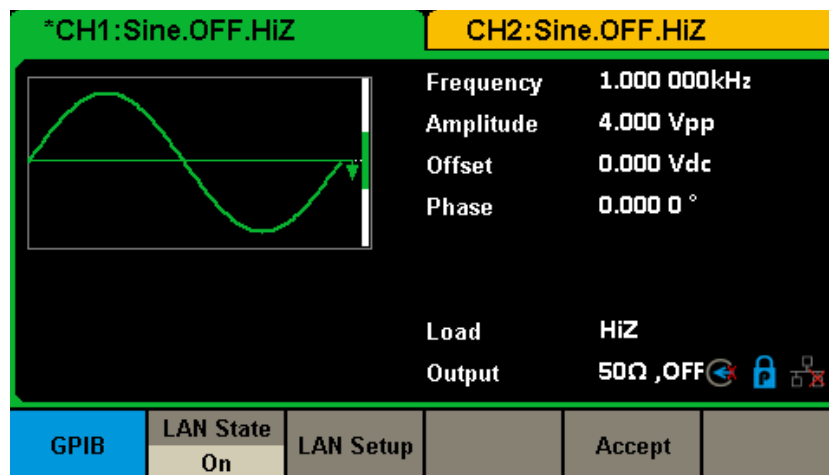
Figure 2-78 Interface Settings
