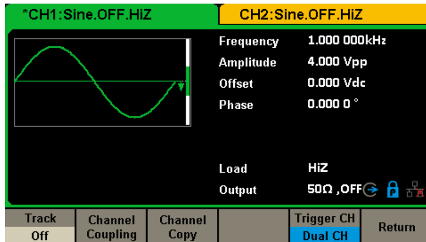
Figure 2-77 Channel trigger signal correlation
