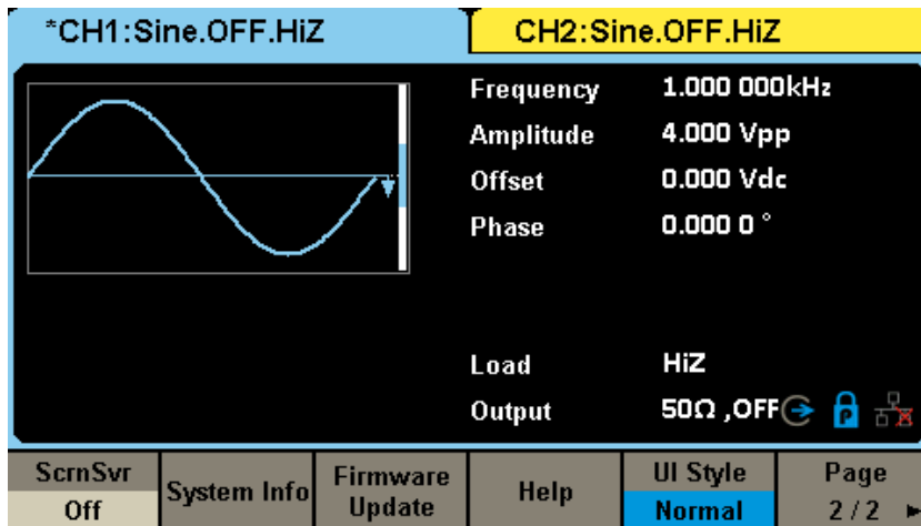
Figure 2-53 Normal UI Style
