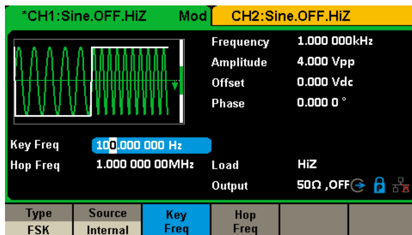
Figure 2-28 Setting Interface of FSK Modulation
