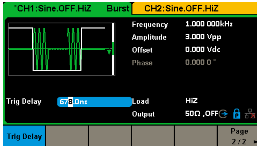
Figure 2-42 Gated Burst Interface (Page 2/2)
