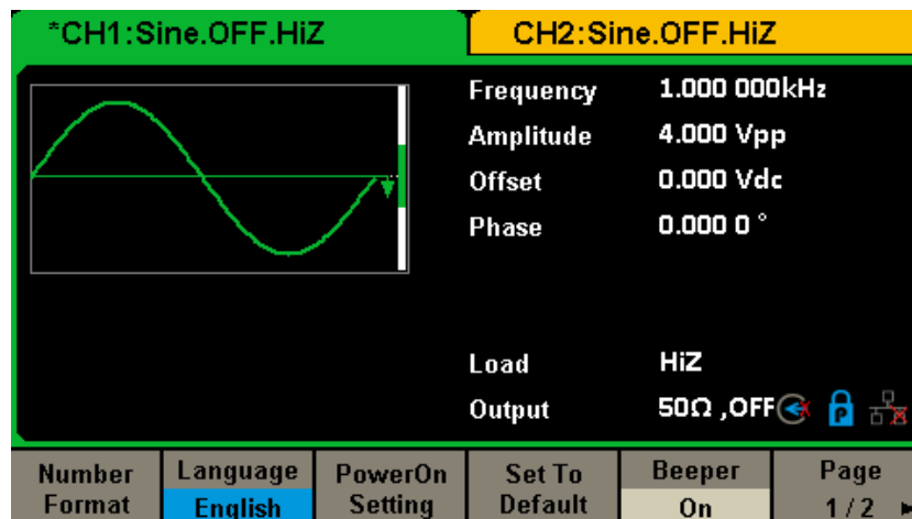
Figure 2-55 English Interface
