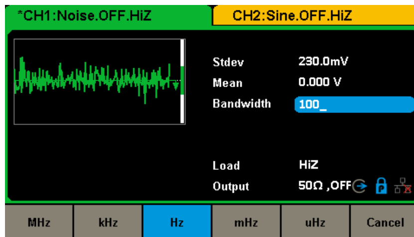
Figure 2-16 Setting the Bandwidth
