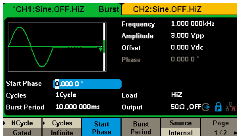
Figure 2-38 N-Cycle Burst Interface (Page 1/2)
