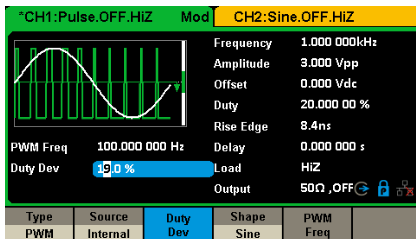
Figure 2-33 Duty Deviation Setting Interface
