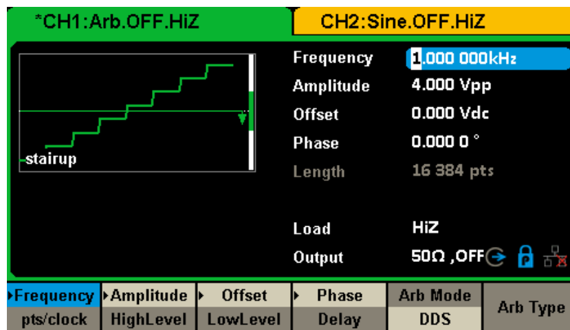
Figure 2-18 Arb Parameters Display Interface (DDS)
