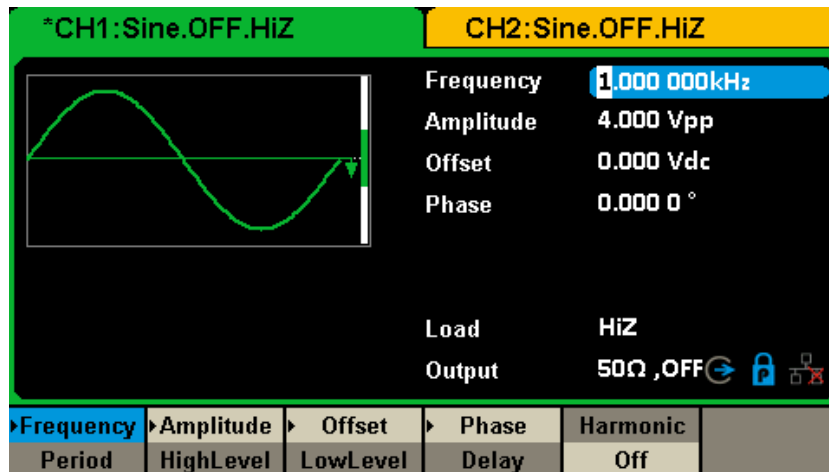
Figure 2-83 Phase-locked Mode
