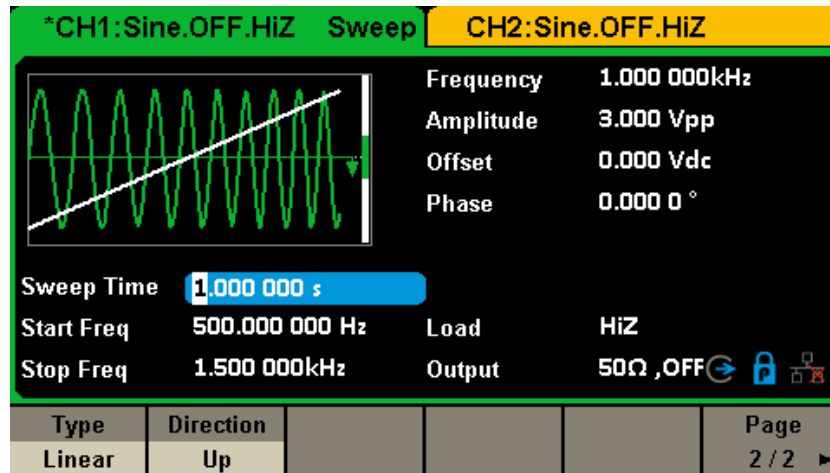
Figure 2-35 Setting Interface of Sweep (Page 2/2)
