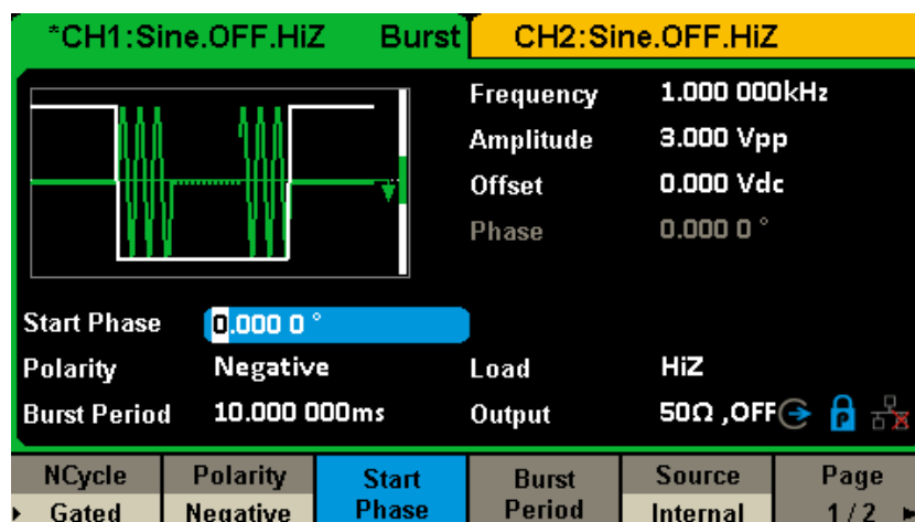
Figure 2-41 Gated Burst Interface (Page 1/2)
