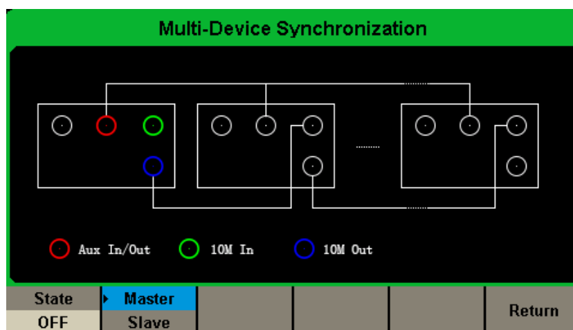
Figure 2-86 Multi-Device Sync Interface
