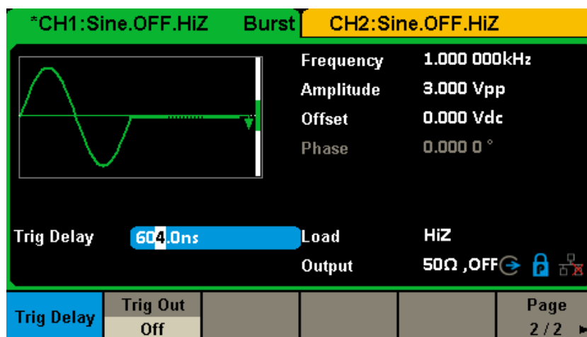
Figure 2-39 N-Cycle Burst Interface (Page 2/2)
