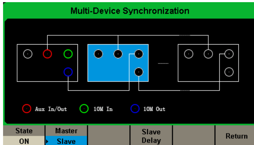
Figure 2-88 Slave mode Interface
