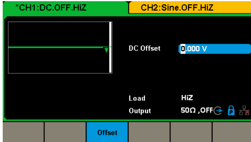
Figure 2-17 DC Setting Interface
