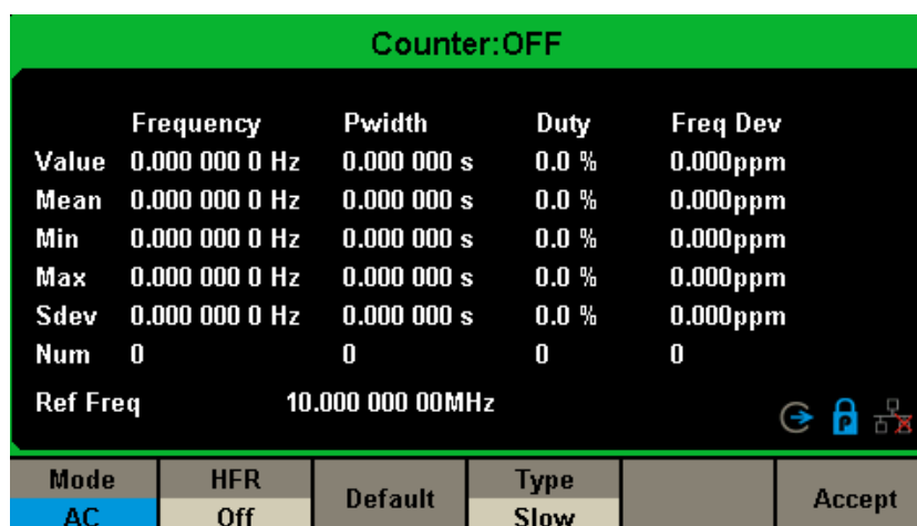
Figure 2-68 Counter Setup Interface
