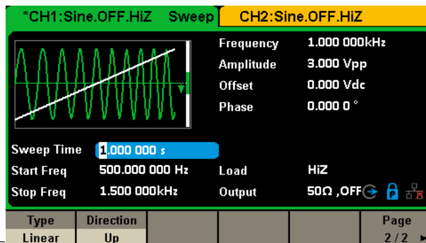
Figure 2-36 Linear Sweep Interface
