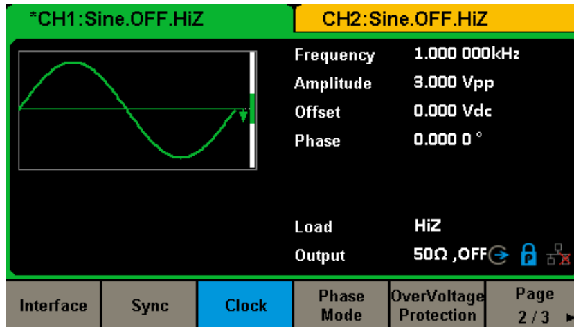
Figure 2-48 Utility Setup Interface (Page 2/3)
