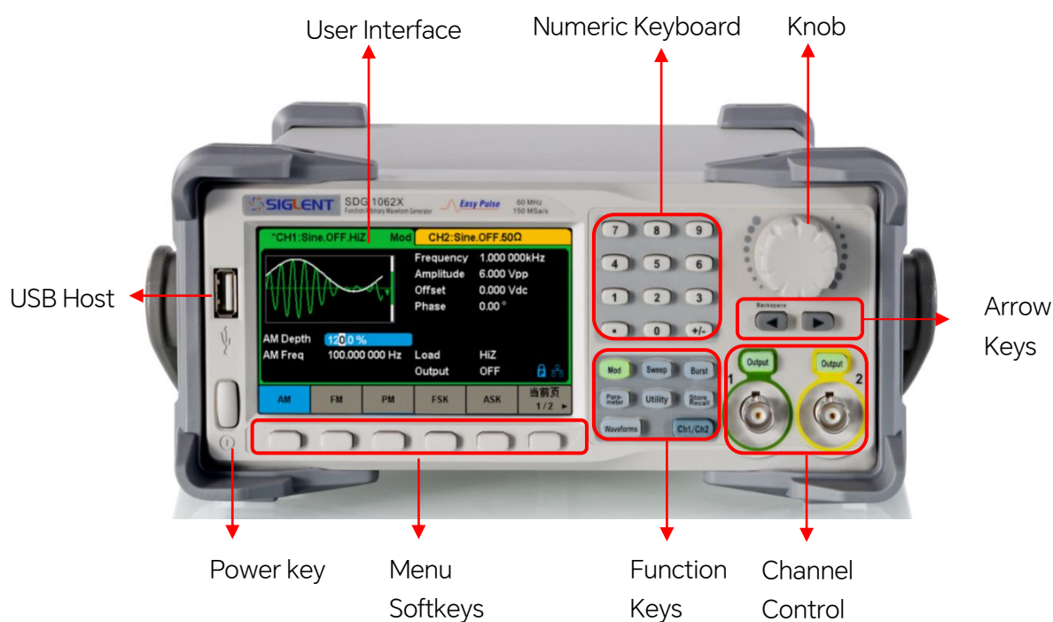
Figure 1-2 Front Panel of SDG2000X
