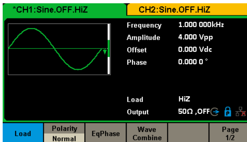
Figure 2-69 Output Setup Interface
