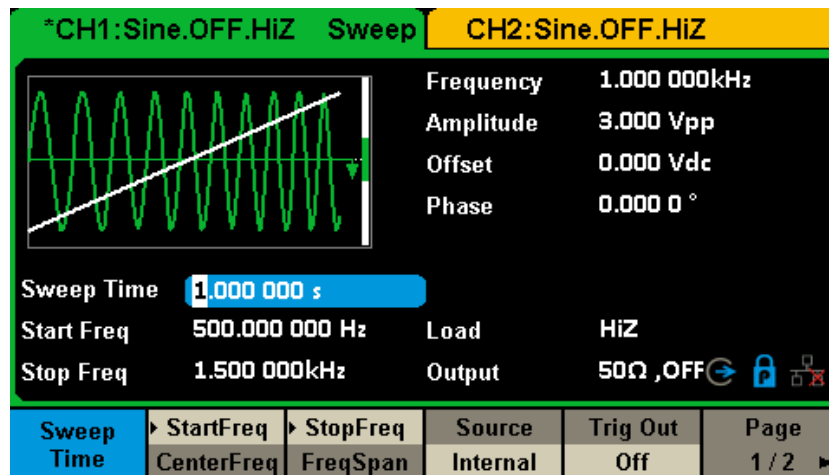
Figure 2-34 Setting Interface of Sweep (Page 1/2)
