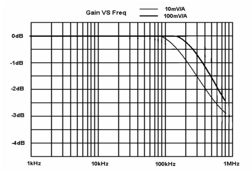
Figure 1 CPL5100 Typical Gain VS Frequency curve
