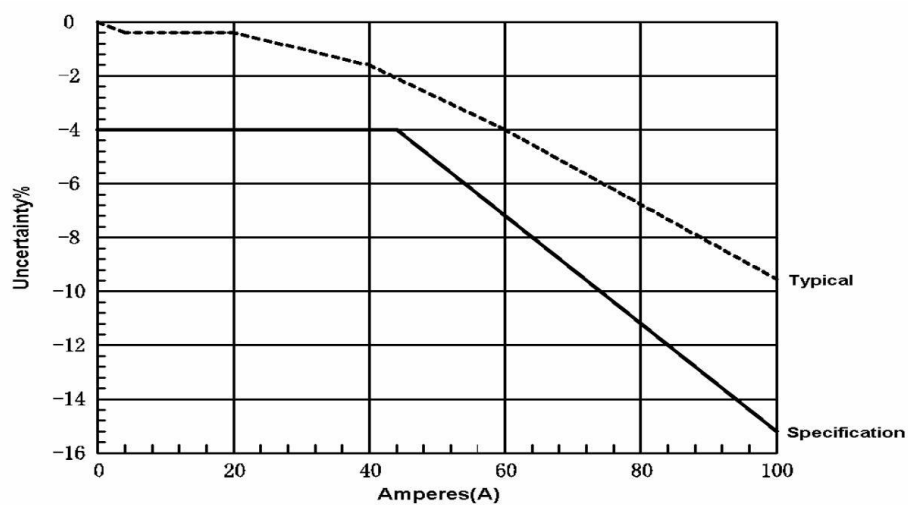
Figure 3 Typical DC linearity (0.01V/A level)
